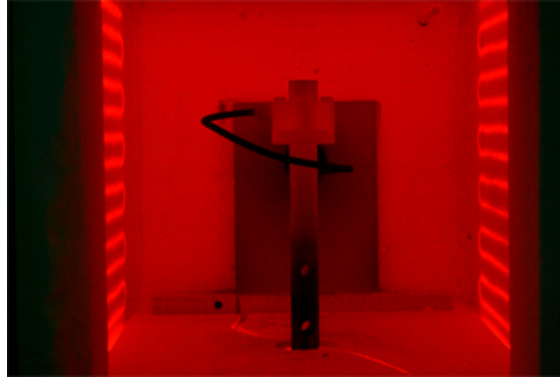
Figure 1 High-temp Accelerometer During Vibration at 1400 °F (760 °C)
