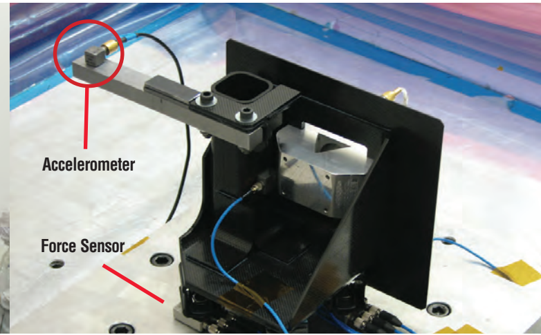
PCB® Model 356M208 accelerometer & force sensors used during vibration testing of bracket assembly at Utah State Space Dynamics Lab
