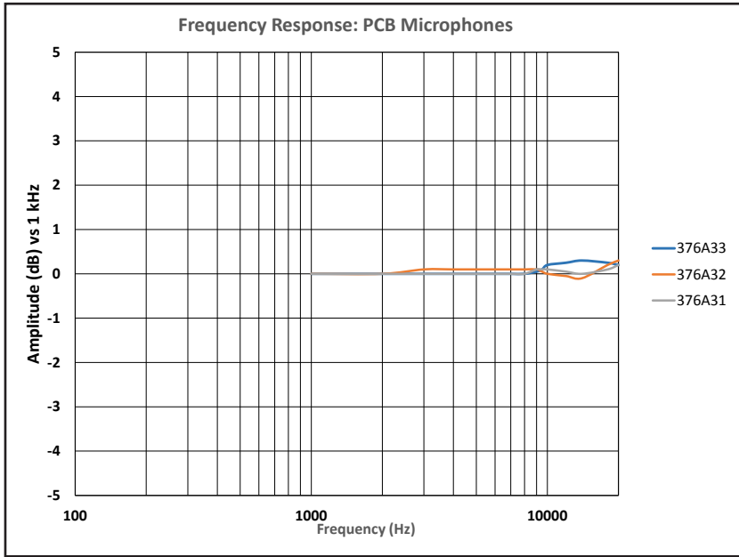
Figure 1: The on-axis frequency responses of the PCB microphones above 1 kHz are within 0.5 dB of flat, and correspond well to the supplied calibration curves.
