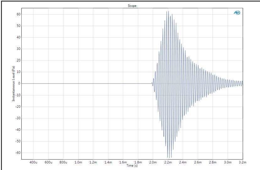
Figure 5: Measurement of the time domain acoustic signal generated by the ultrasonic module demonstrates the bandwidth and the high SPL capability of the 376A31 mic.
