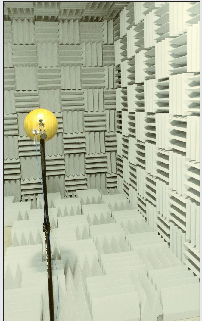
Photo 5: Calibration and development are validated in a custom-built anechoic chamber. (Photo courtesy of PCB Piezotronics)
