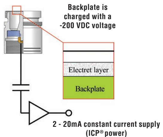
Prepolarized
