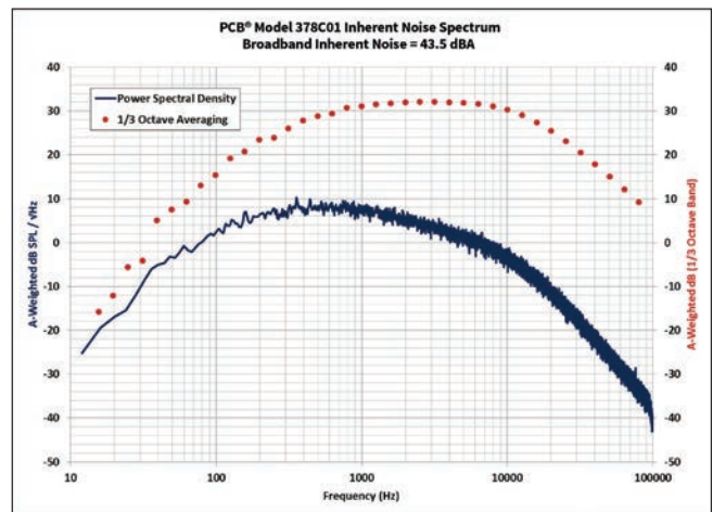
1/4" Microphone, A-weighted
