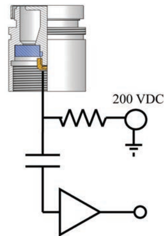
Externally Polarized
