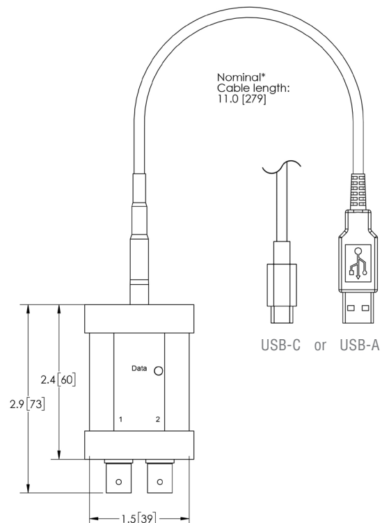
DigiDAQ™ Outline Drawing Dimensions in inches [mm]
