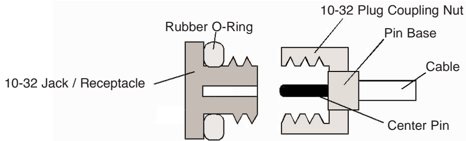
Anatomy of a typical connection between a 10-32 connectors
