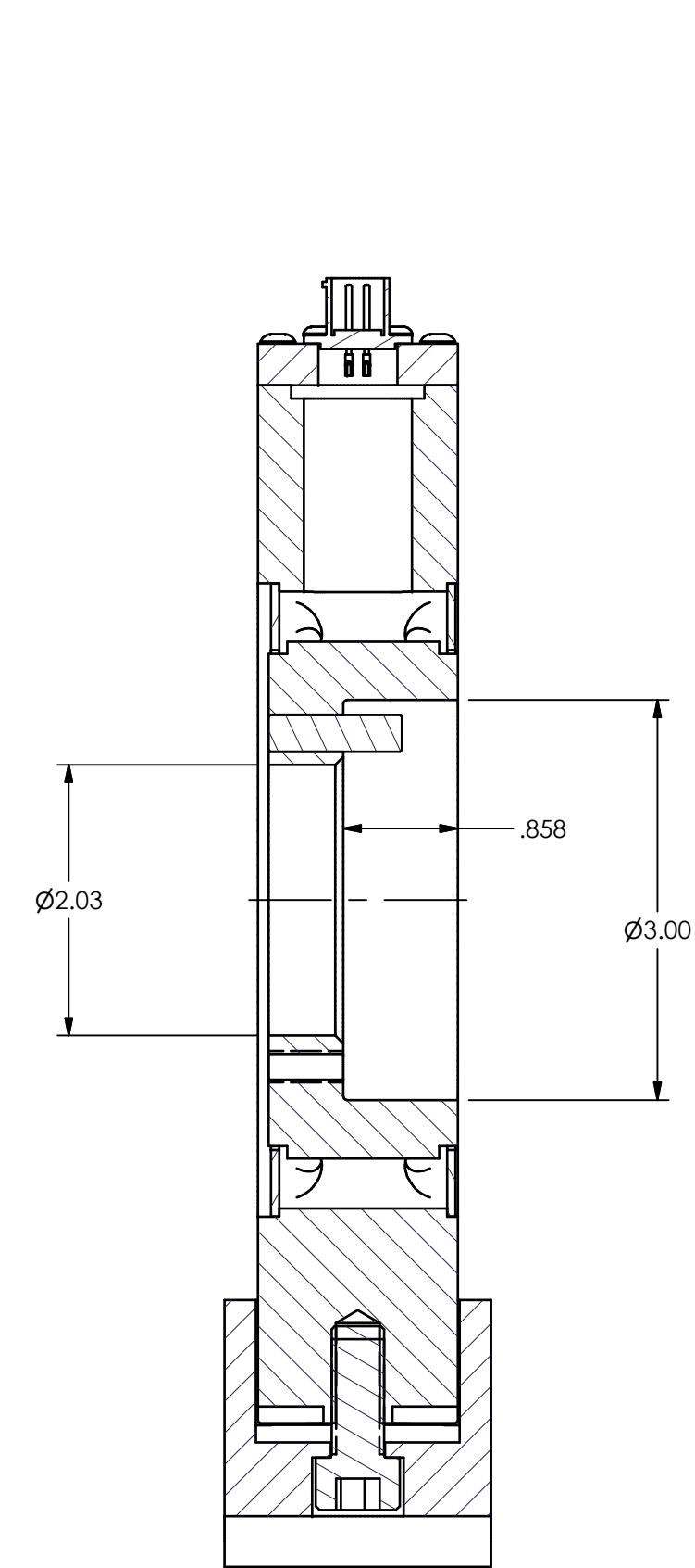
SECTION A-A SCALE 3/4
