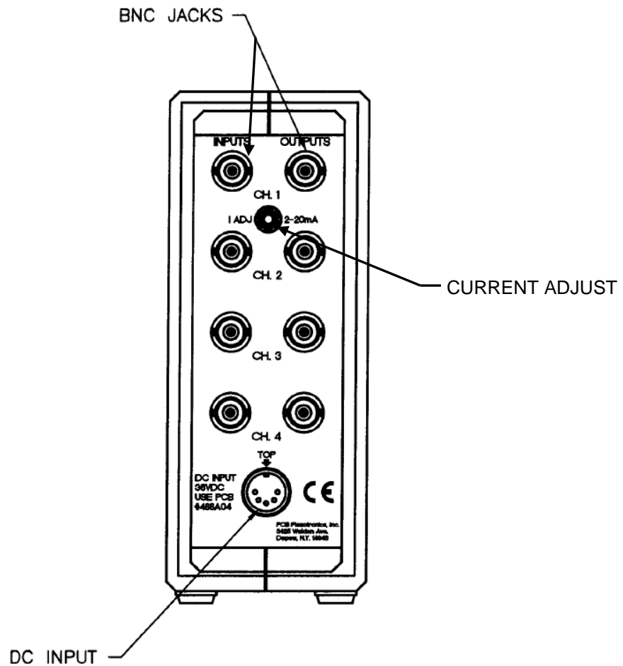
Figure 3: Constant Current Adjust
