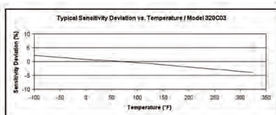
Model 320C03
