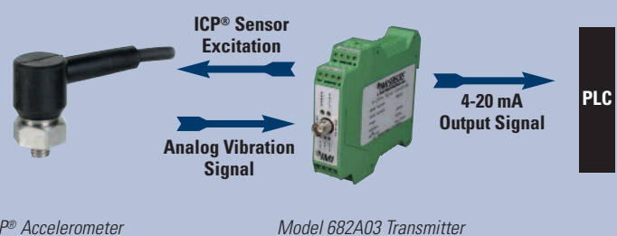
ICP® Accelerometer
